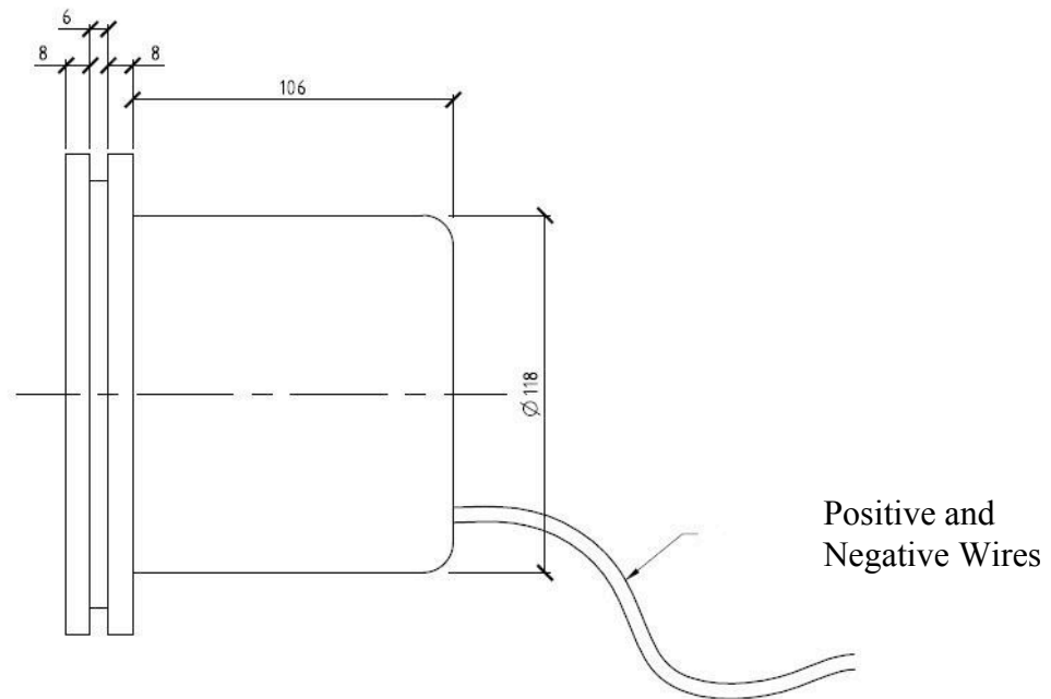
SIDE VIEW
